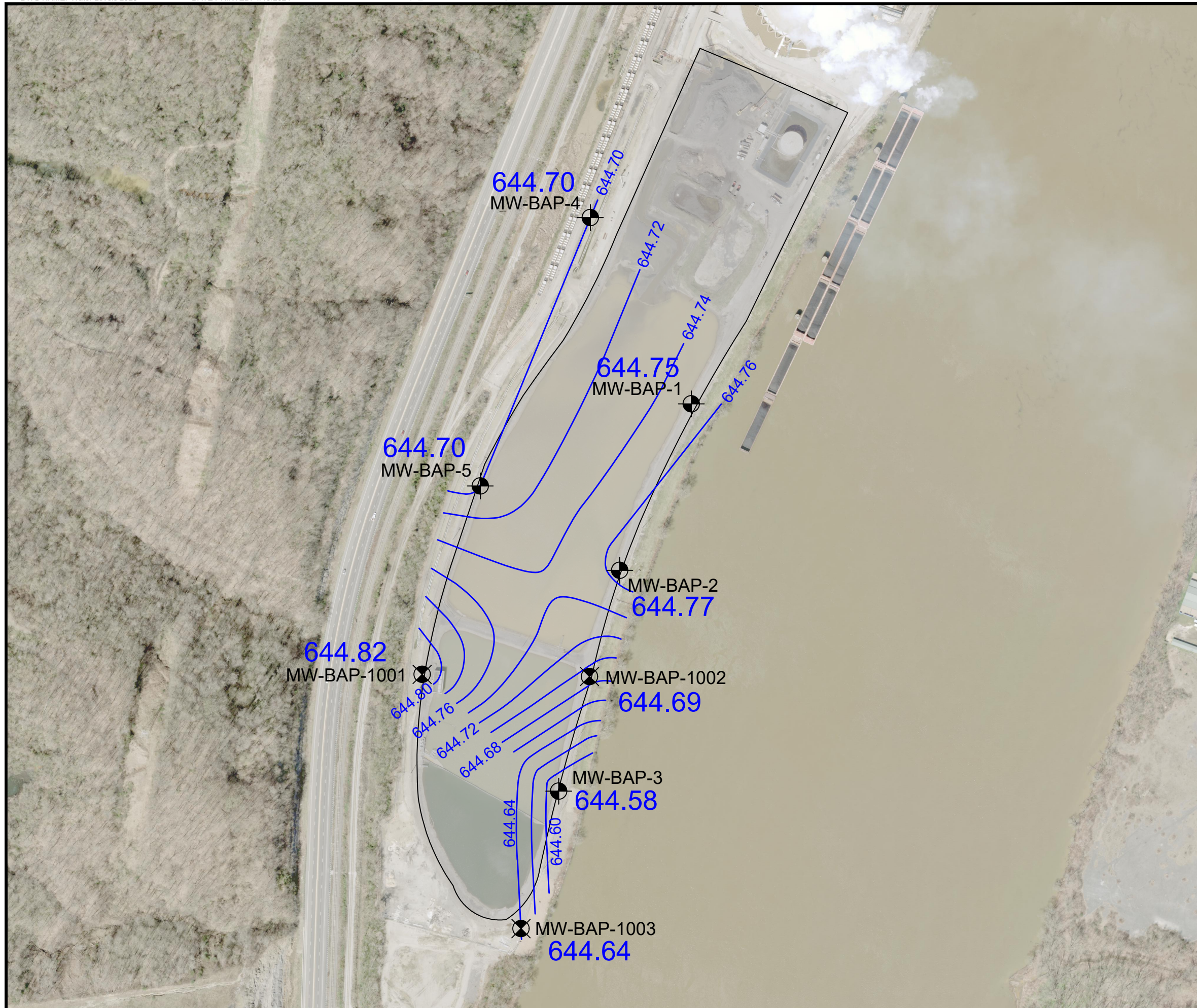
Potentiometric Surface Map - Uppermost Aquifer - October 9, 2023, Bottom Ash Pond (BAP), Cardinal Plant, Brilliant, Ohio
